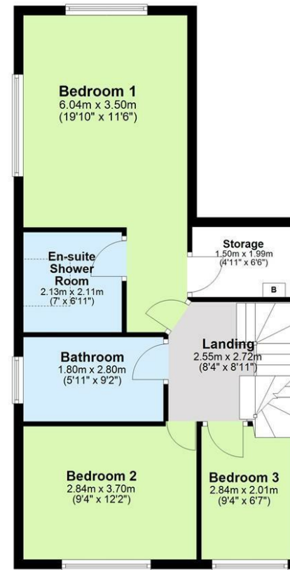
First Floor Approx. 56.3 sq. metres (606.3 sq. feet)
