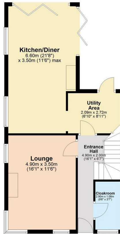
Ground Floor Approx. 56.4 sq. metres (607.0 sq. feet)
